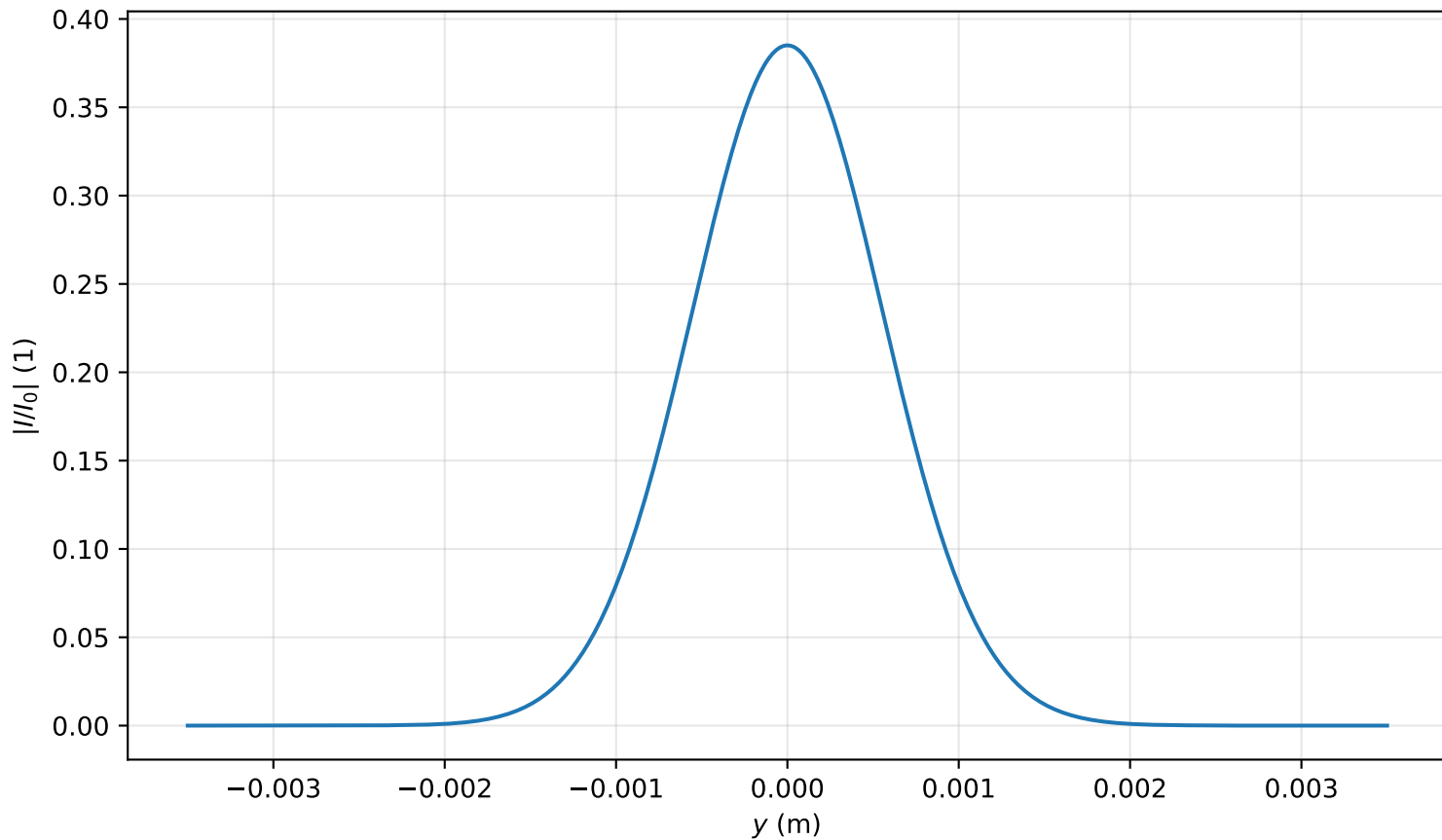
Intensity profile I(x = 0, y, z = 2.707)/I_0 , P_{in}=0.1P_{cr} , artificial time
